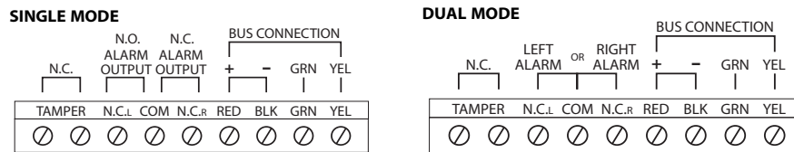
Figure 1: Wiring Methods
